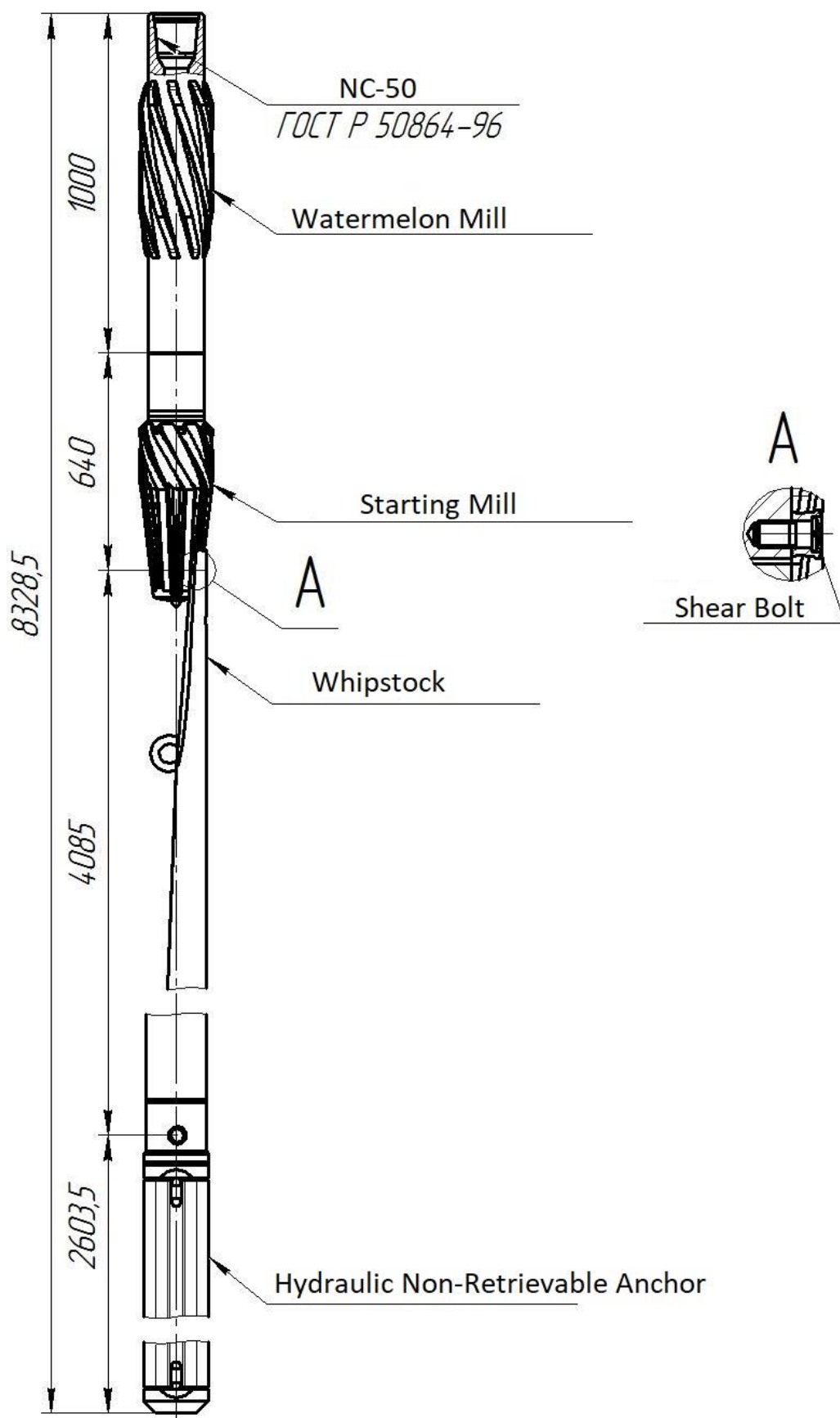
Fig. 1 - Sketch of Whipstock set hydraulic non-retrievable 9-5/8" Ø 245 mm.
